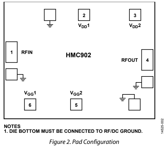
Figure 2. Pad Configuration
