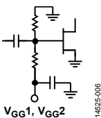
Figure 6. V GG1 , V GG2 Interface Schematic
