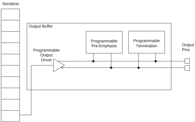
Figure 2–6. Output Buffer
