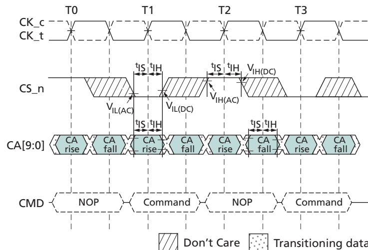
Figure 20: Command and Input Setup and Hold
