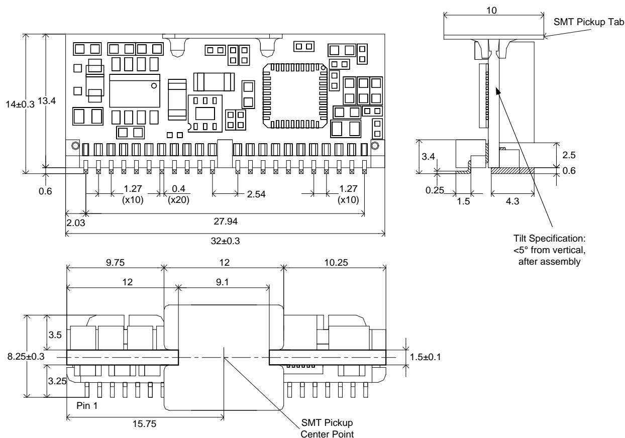
Figure 60. Mechanical Drawing
