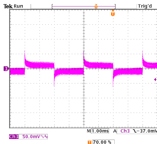
Figure 53. Transient Response with Regulation set to 0.74 mV/A
