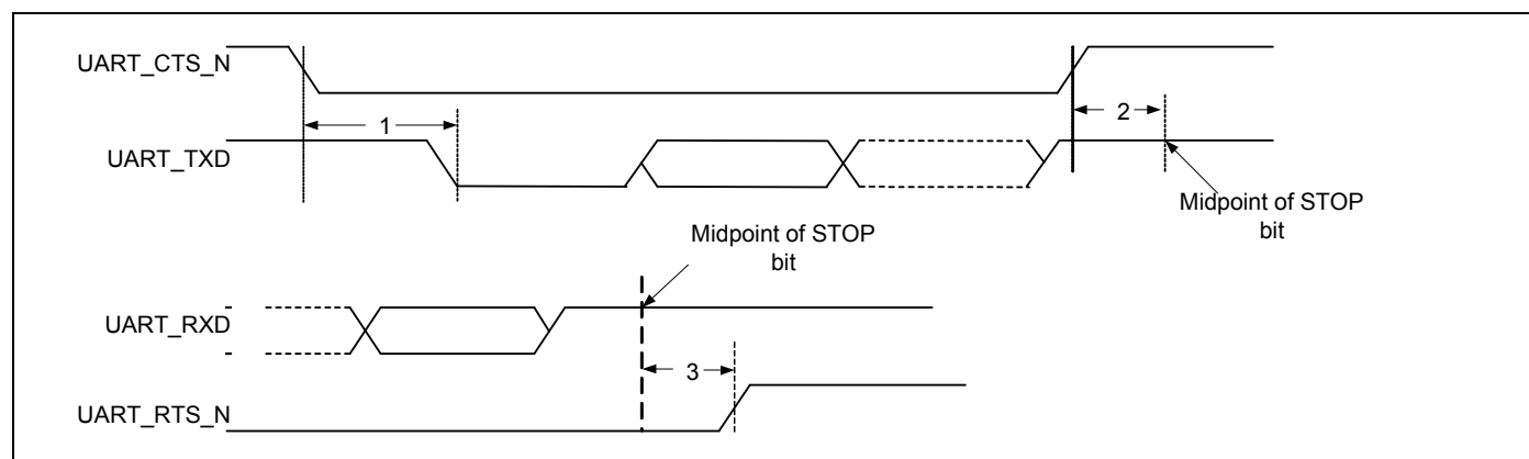
Figure 12. UART Timing
