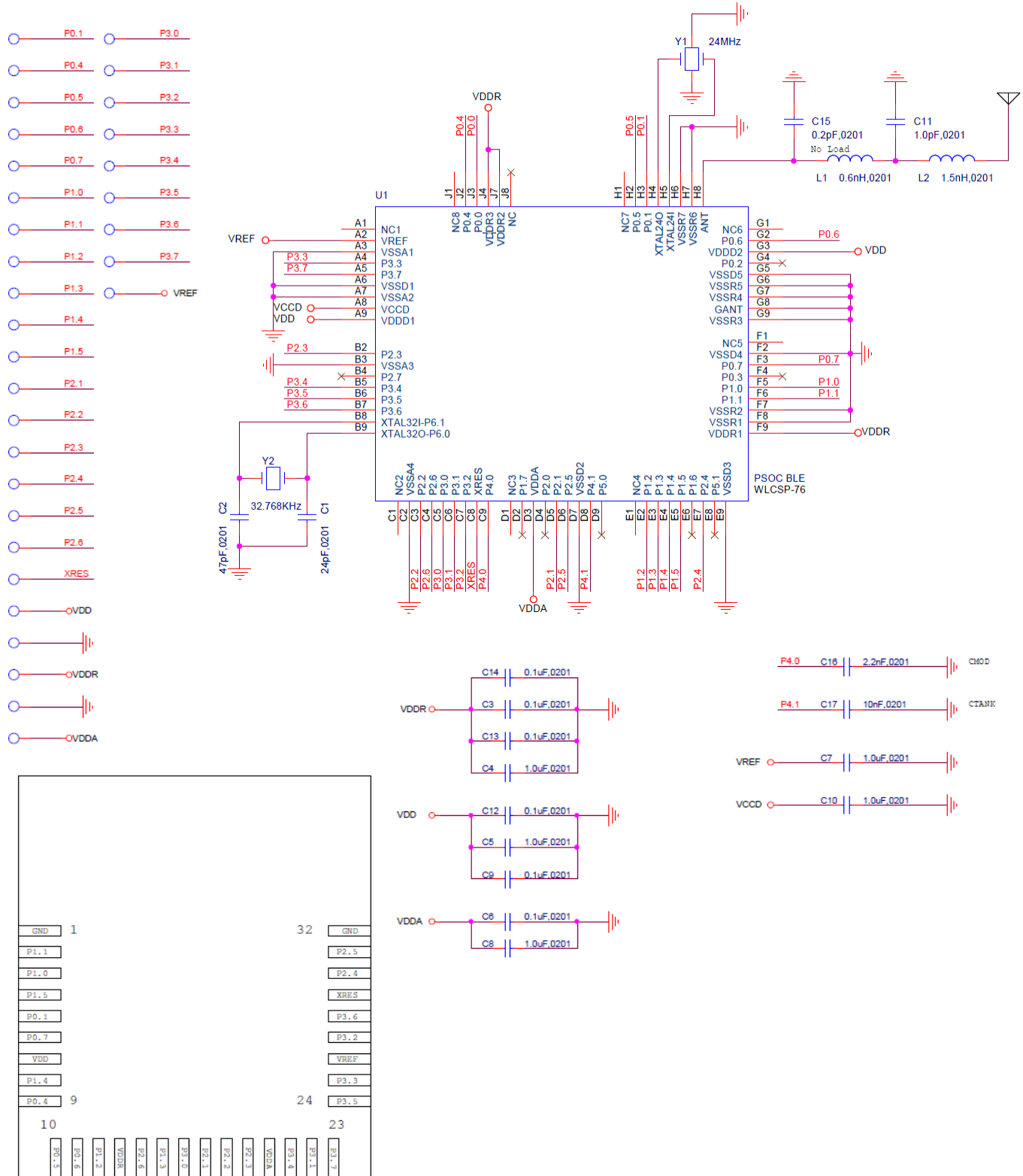
Figure 9. CYBLE-214009-00 Schematic Diagram
