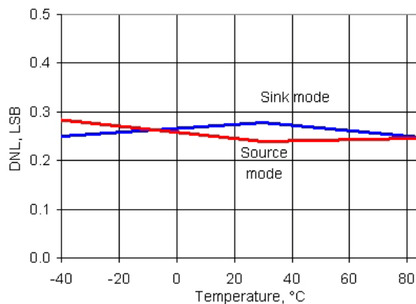
Figure 11-38. IDAC DNL vs Temperature, Range = 255 \mu A, High speed mode
