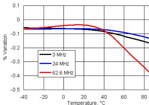
Figure 11-70. IMO Frequency Variation vs. Temperature
