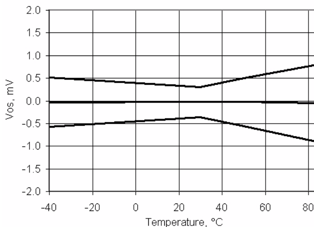
Figure 11-25. Opamp Voffset vs Temperature, V_{DDA} = 5\text{ V}
