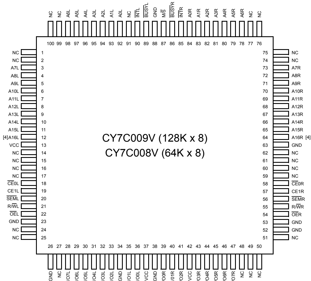
100-Pin TQFP (Top View)
