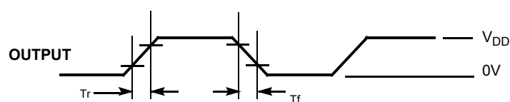
Figure 4. Output Rise/Fall Time (SSCLK and REFCLK)
