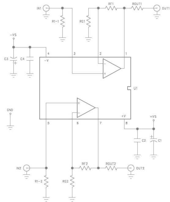
Figure 13. CEB006 &amp; CEB010 Schematic
