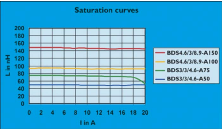
Figure 57. Saturation Curves gapped SMD beads
