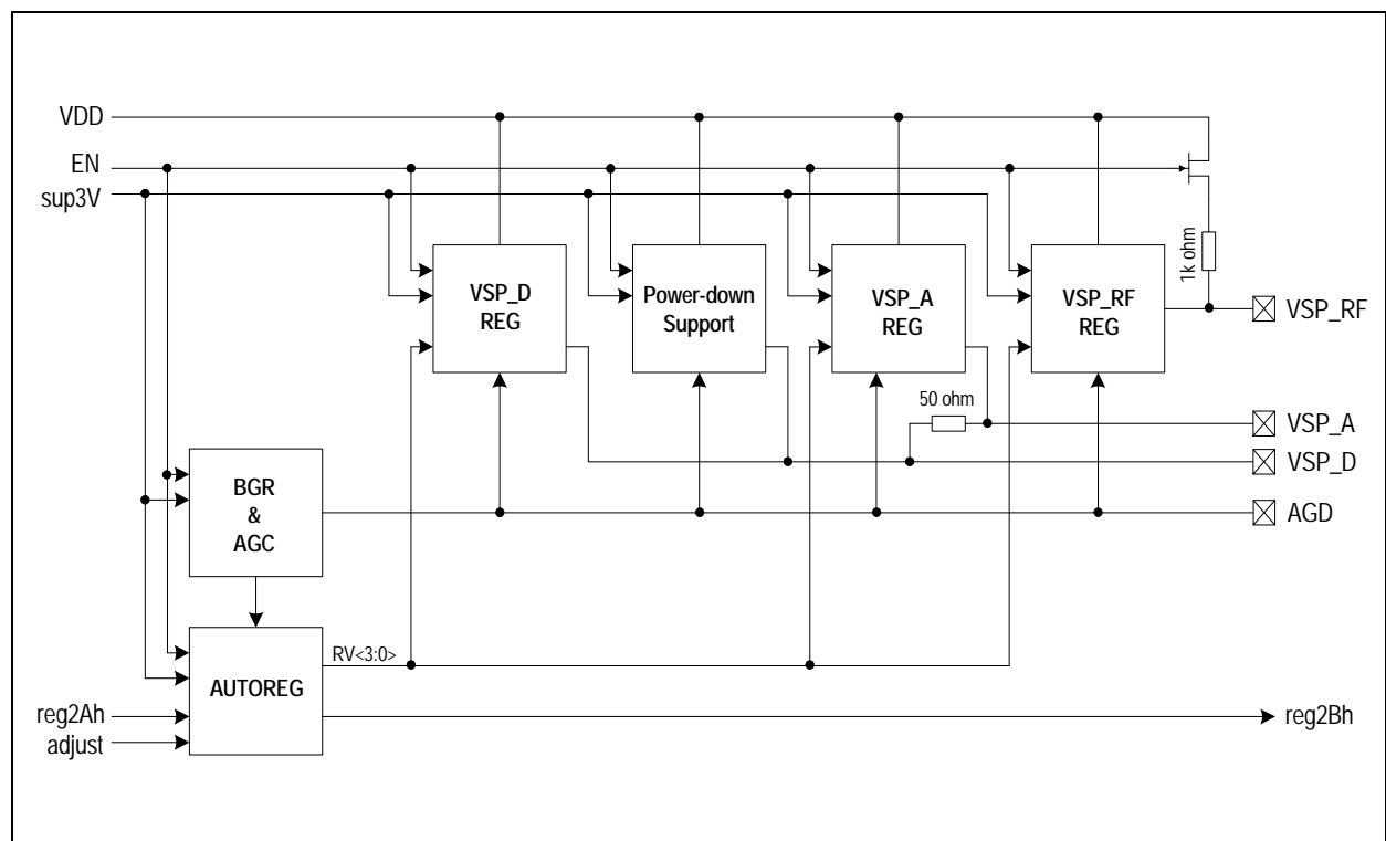
Figure 22: The AS3911 Power Supply System
