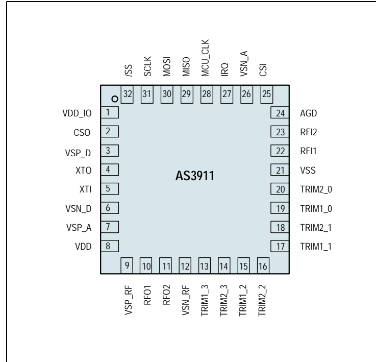
Figure 3: Pin Diagram
