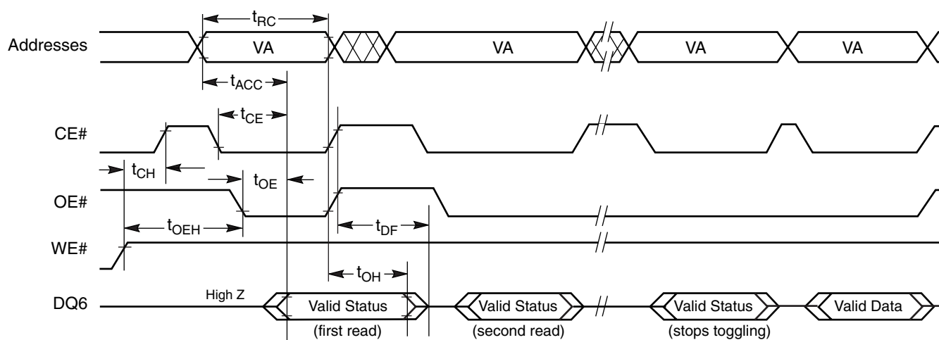
Figure 12. Toggle Bit Timings (During Embedded Algorithms)
