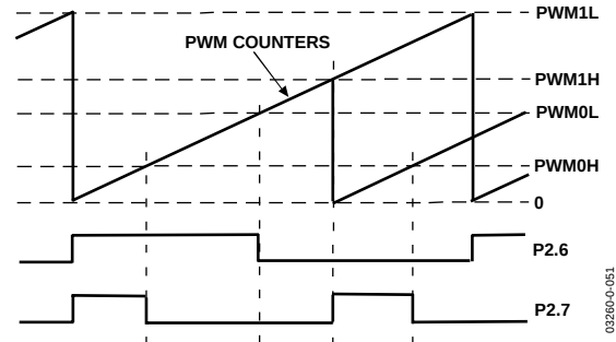
Figure 52. PWM Mode 5
