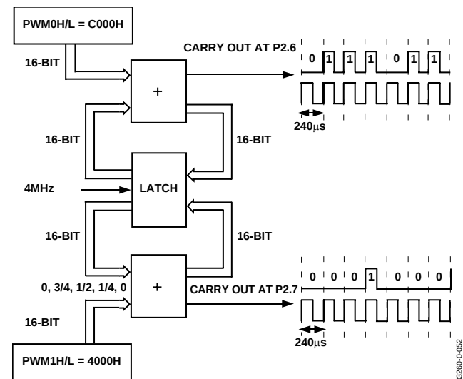
Figure 53. PWM Mode 6
