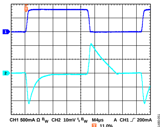
Figure 51. Output Transient Response, V_{OUT} = 5\text{ V} , C_{OUT} = 10\text{ }\mu\text{F}
