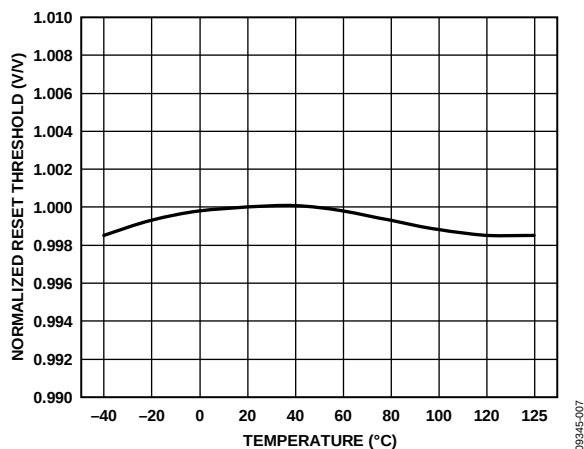
Figure 7. Reset Threshold vs. Temperature
