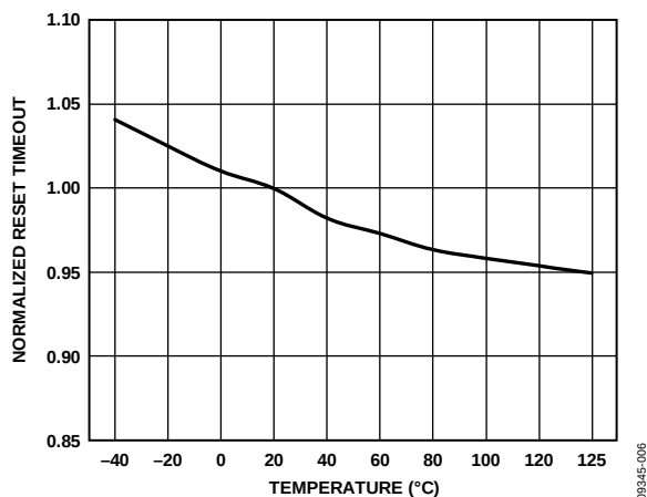
Figure 6. Reset Timeout vs. Temperature
