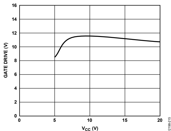
Figure 15. GATE Drive vs. V CC
