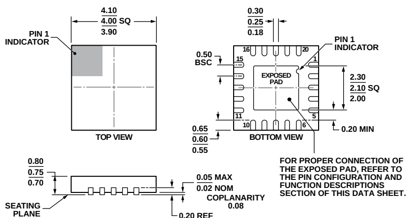
Figure 31. 20-Lead Lead Frame Chip Scale Package [LFCSP_WQ] 4 mm × 4 mm Body, Very Very Thin Quad (CP-20-6)
