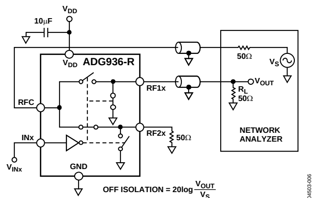
Figure 21. Off Isolation
