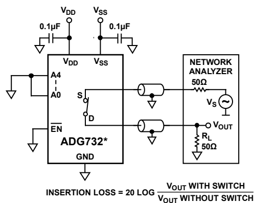
Figure 26. Bandwidth
