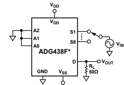
*SIMILAR CONNECTION FOR ADG439F. Figure 23. Off Isolation
