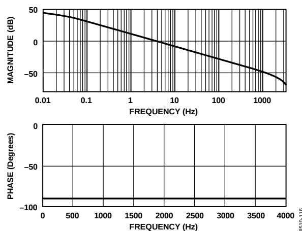
Figure 39. Combined Gain and Phase Response of the Digital Integrator
