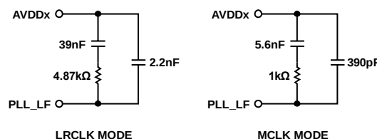
Figure 15. PLL Filter
