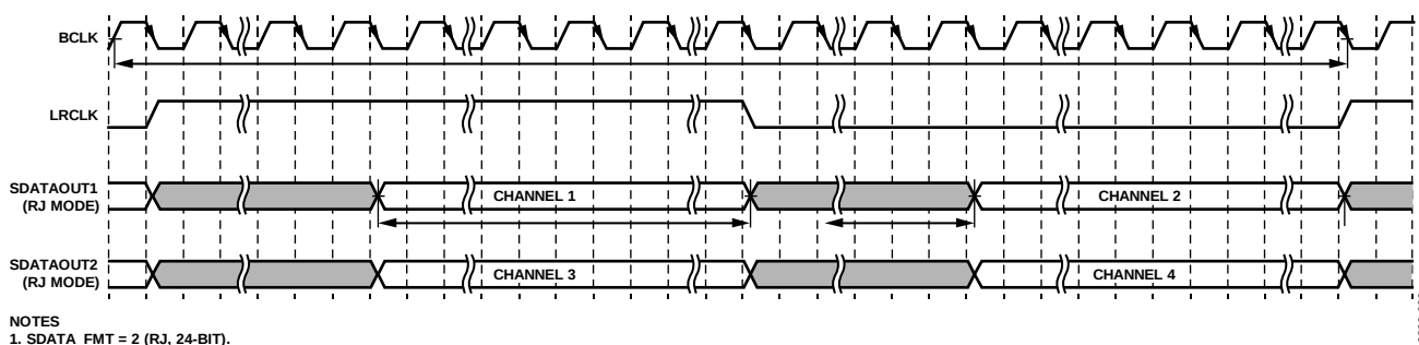
Figure 26. RJ Audio Format
