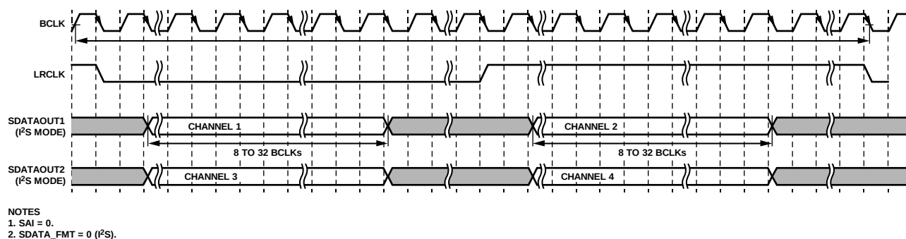
Figure 24. I 2 S Audio Format
