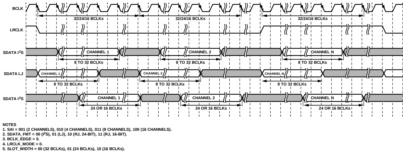
Figure 27. TDM Nonpulse Mode Audio Format
