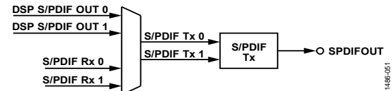
Figure 48. S/PDIF Transmitter Source Selection
