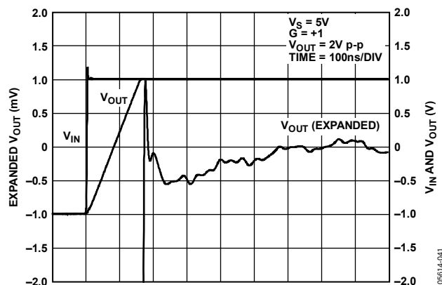
Figure 28. Settling Time
