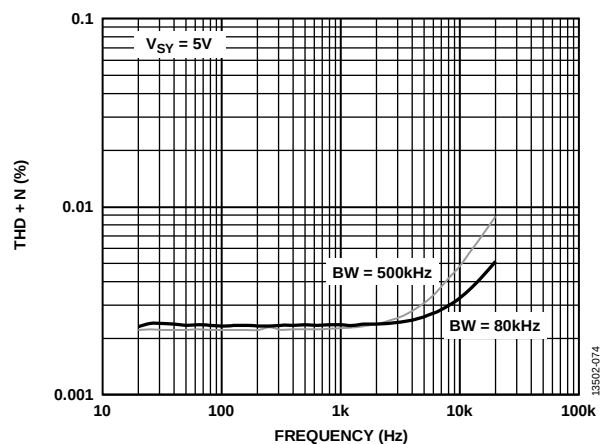
Figure 78. THD + N vs. Frequency, V_{SV} = 5\text{ V}
