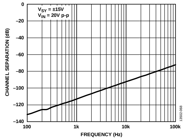
Figure 72. Channel Separation vs. Frequency, V_{SY} = \pm 15\text{ V}
