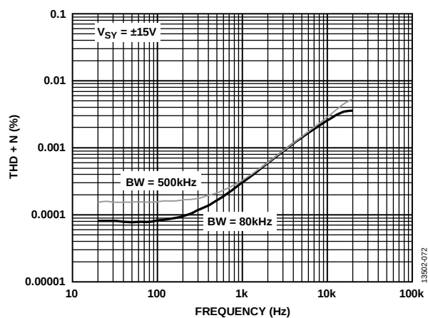
Figure 76. THD + N vs. Frequency, V_{SV} = \pm 15\text{ V}
