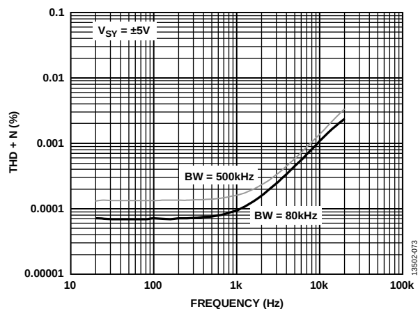
Figure 77. THD + N vs. Frequency, V_{SV} = \pm 5\text{ V}
