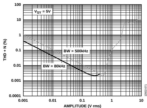
Figure 75. THD + N vs. Amplitude, V_{SV} = 5\text{ V}
