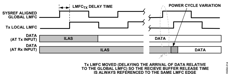
Figure 144. Adjusting the JESD204B Tx LMFC in the AD9689
