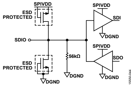
Figure 73. SDIO Input
