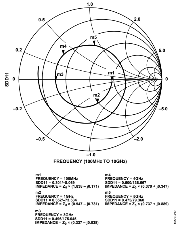
Figure 78. Differential Input Return Loss
