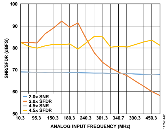
Figure 90. SNR/SFDR vs. f_{IN} ; f_{IN} < 500 \text{ MHz} ; Buffer Control 1 (0x018) = 2.0x and 4.5x
