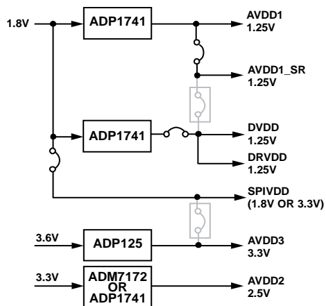
Figure 185. High Efficiency, Low Noise Power Solution for the AD9680
