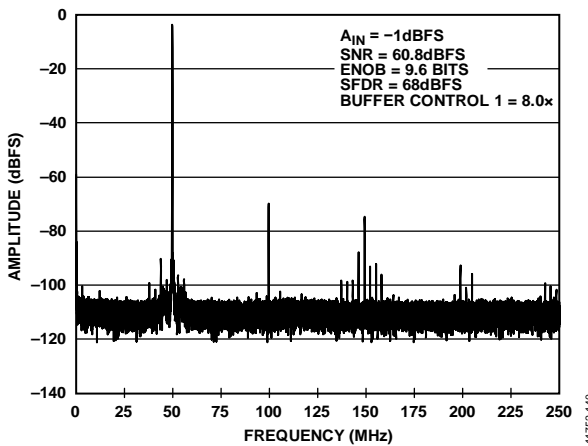
Figure 88. Single-Tone FFT with f_{IN} = 1950.3 \text{ MHz}
