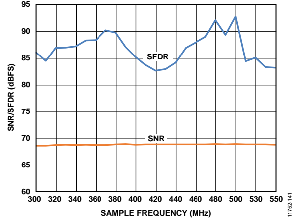
Figure 89. SNR/SFDR vs. f_s , f_{IN} = 170.3 \text{ MHz} ; Buffer Control 1 = 2.0x
