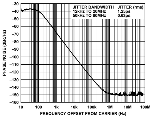
Figure 5. Phase Noise ( f_{REF} = 61.44 MHz, f_{OUT1} = 122.88 MHz)
