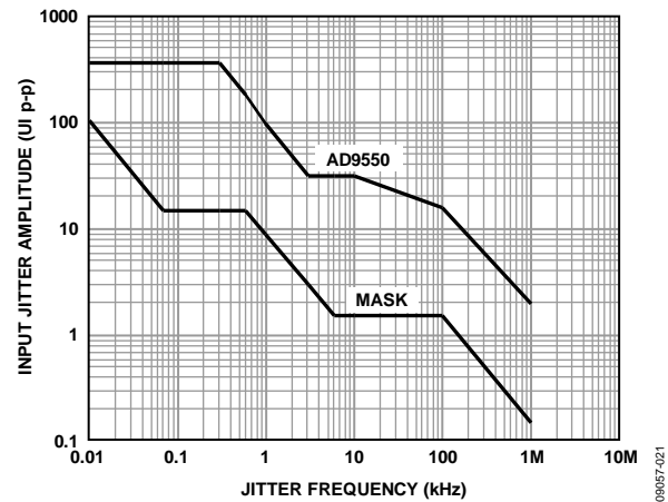
Figure 25. Jitter Tolerance
