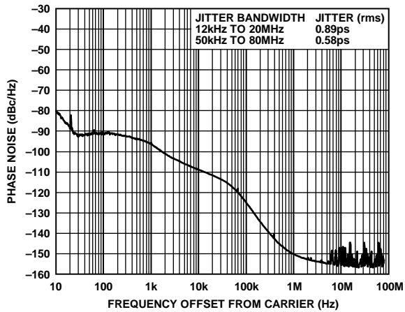
Figure 3. Phase Noise ( f_{REF} = 25 MHz, f_{OUT1} = 125 MHz)
