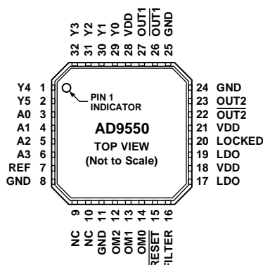
Figure 2. Pin Configuration
