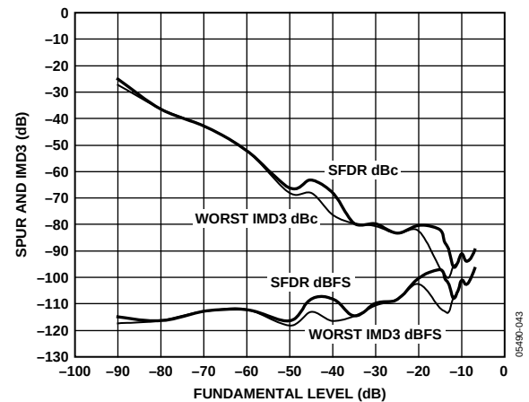
Figure 41. AD9446-80 Two-Tone SFDR vs. Analog Input Level 80 MSPS/ 9.8 MHz, 10.8 MHz
