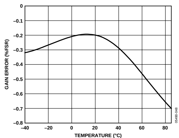
Figure 46. AD9446-100 Gain vs. Temperature
