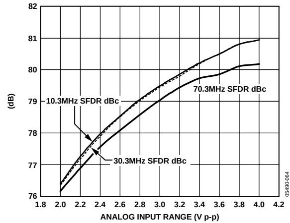
Figure 51. AD9446-100 SNR vs. Analog Input Range, 100 MSPS
