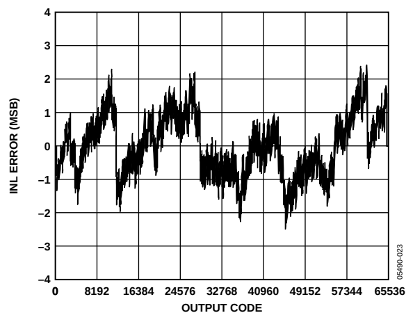
Figure 23. AD9446-80 INL Error vs. Output Code, 80 MSPS, 10.3 MHz
