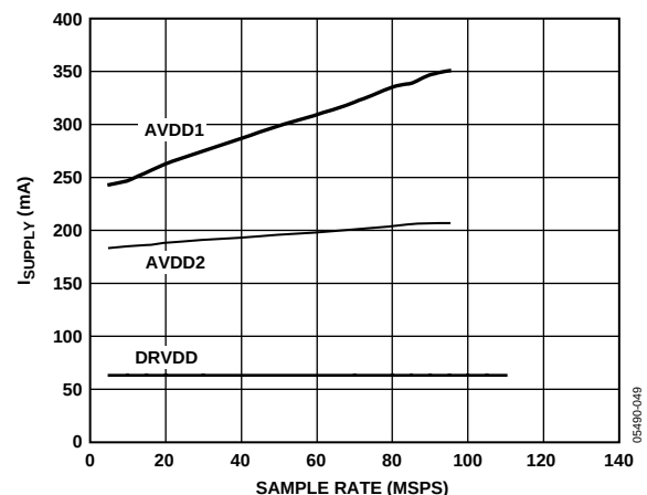
Figure 47. AD9446-80 Power Supply Current vs. Sample Rate 10.3 MHz @ -1 dBFS
