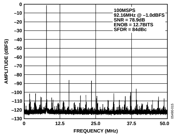
Figure 15. AD9446-100 64k Point Single-Tone FFT/100 MSPS/92.16 MHz
