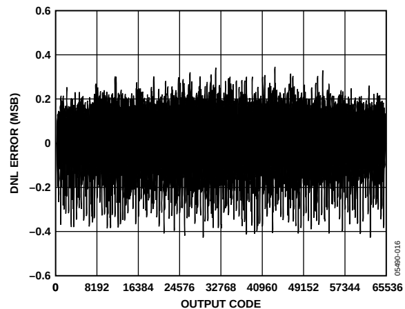
Figure 16. AD9446-100 DNL Error vs. Output Code, 100 MSPS, 10.3 MHz
