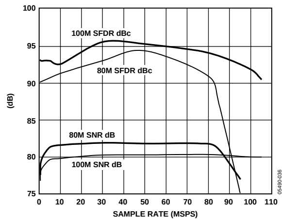
Figure 54. AD9446 Single-Tone SNR/SFDR vs. Sample Rate 2.3 MHz
