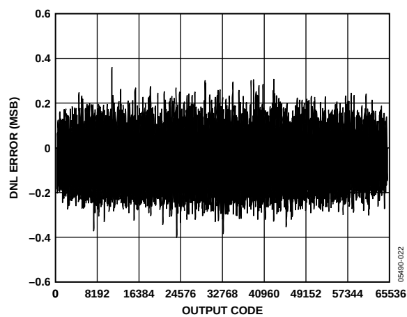
Figure 22. AD9446-80 DNL Error vs. Output Code, 80 MSPS, 10.3 MHz
