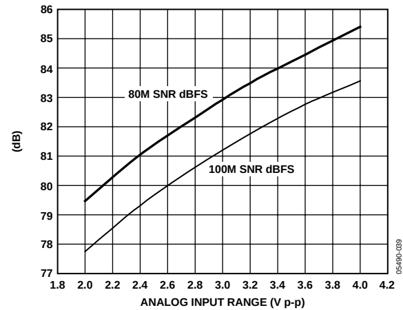
Figure 28. AD9446-100 SNR vs. Input Range, 30.3 MHz, -30 dBFS
