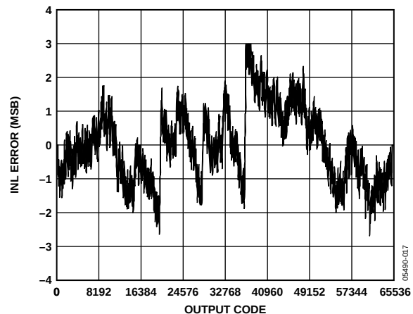
Figure 17. AD9446-100 INL Error vs. Output Code, 100 MSPS, 10.3 MHz
