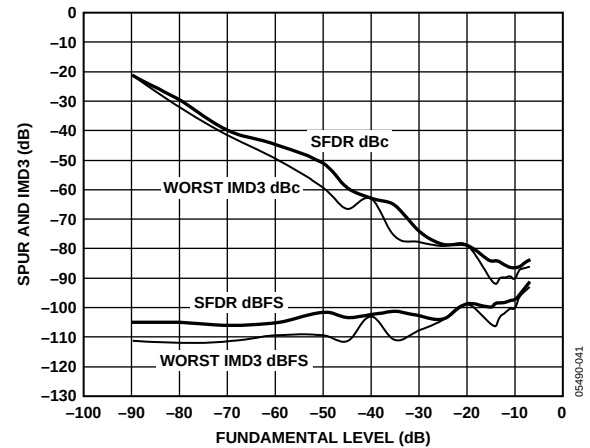
Figure 39. AD9446-100 Two-Tone SFDR vs. Analog Input Level 100 MSPS/ 69.3 MHz, 70.3 MHz
