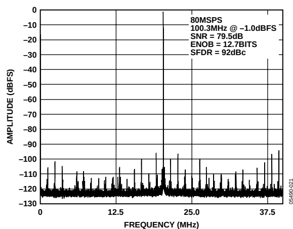
Figure 21. AD9446-80 64k Point Single-Tone FFT/80 MSPS/100.3 MHz
