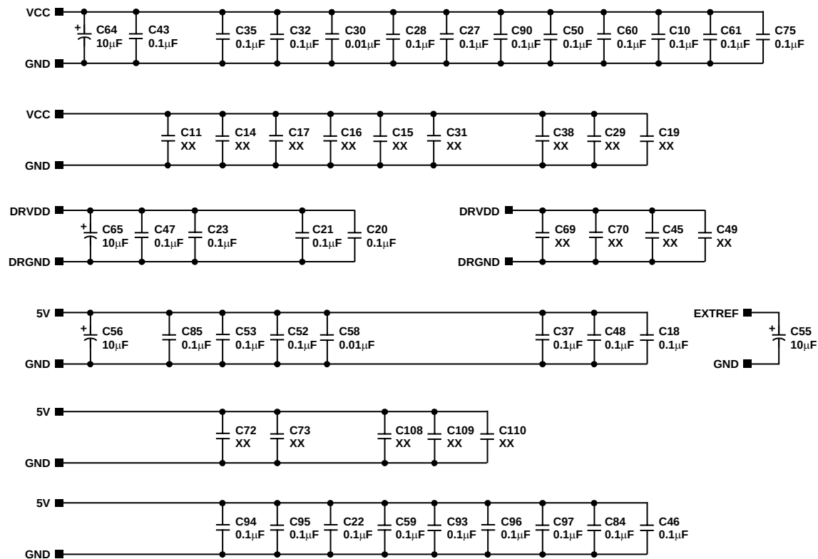
Figure 63. AD9446 Evaluation Board Schematic (Continued)
