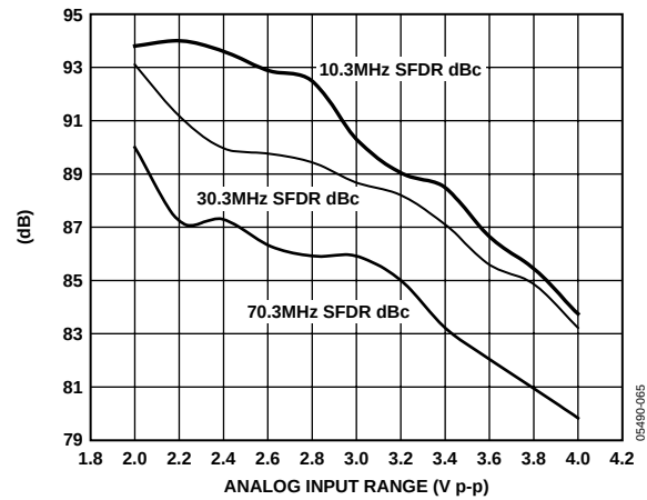
Figure 52. AD9446-80 SFDR vs. Analog Input Range, 100 MSPS
