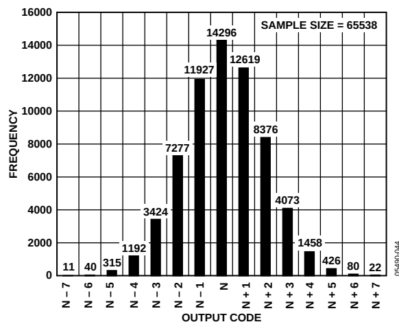
Figure 42. AD9446-100 Grounded Input Histogram
