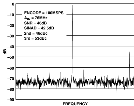
TPC 3. Spectrum: f_S = 100 MSPS, f_{IN} = 76 MHz
