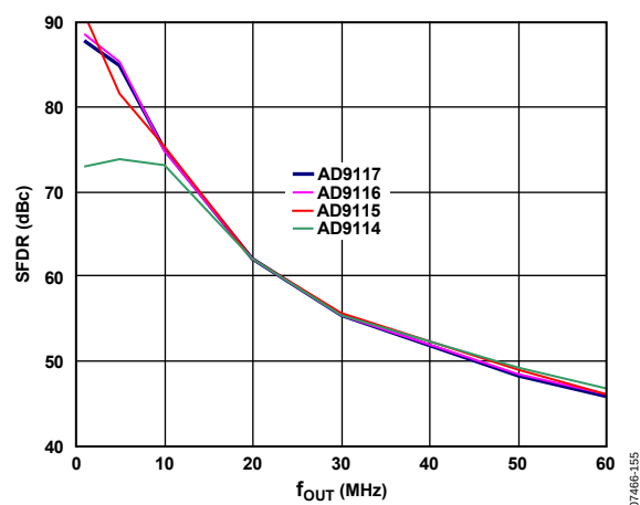
Figure 55. SFDR at 8 mA vs. f_{OUT} , 1.8 V
