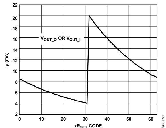
Figure 98. Effect of xR_{SET} Code
