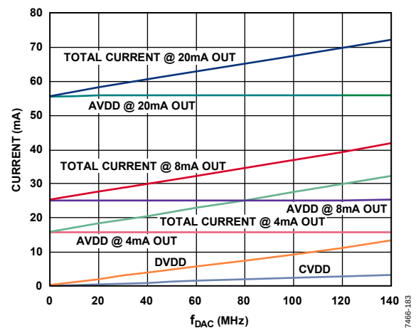
Figure 83. AD9114/AD9115/AD9116/AD9117 Supply Current vs. f_{DAC} , 3.3 V
