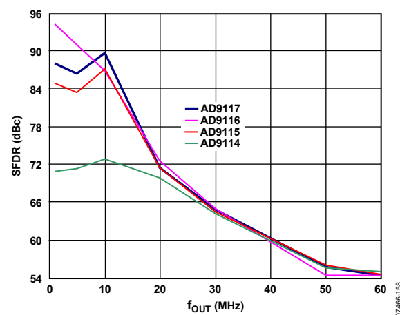
Figure 58. AD9117 SFDR at 20 mA vs. f_{OUT} , 3.3 V
