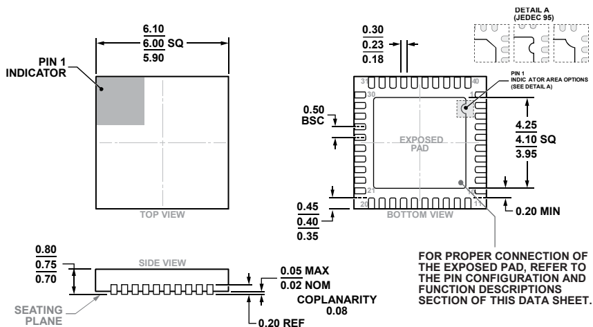
Figure 112. 40-Lead Lead Frame Chip Scale Package [LFCSP]
