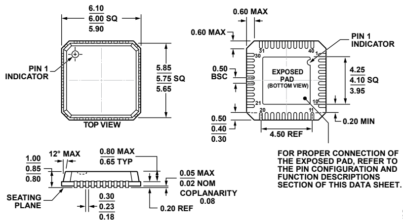
Figure 111. 40-Lead Lead Frame Chip Scale Package [LFCSP]
