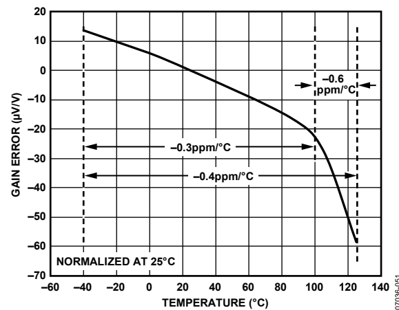
Figure 31. Gain Error vs. Temperature, G = 1
