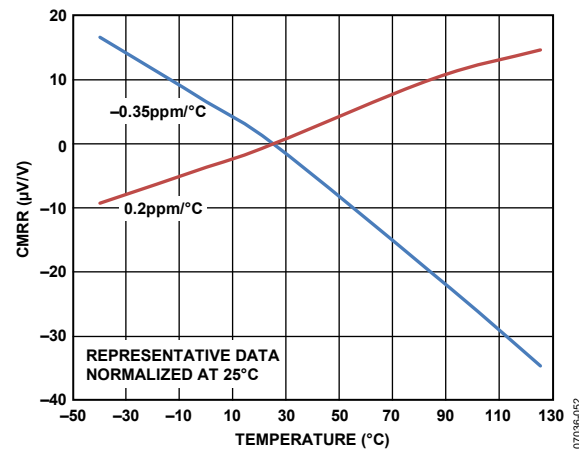
Figure 32. CMRR vs. Temperature, G = 1
