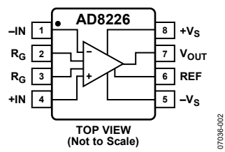
Figure 2. Pin Configuration
