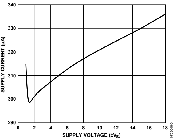
Figure 57. Supply Current vs. Supply Voltage
