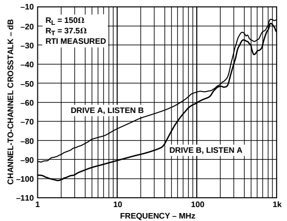
Figure 13. AD8185 Channel-to-Channel Crosstalk vs. Frequency
