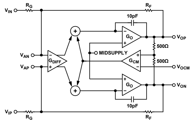
Figure 60. Block Diagram
