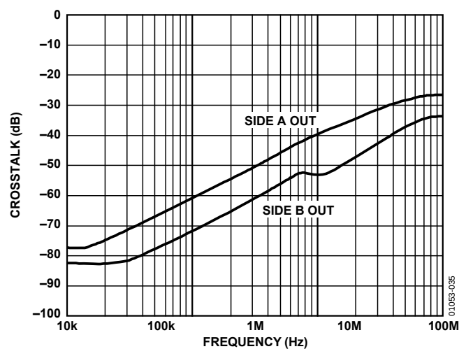
Figure 35. Output-to-Output Crosstalk vs. Frequency, V_S = \pm 12\text{ V}
