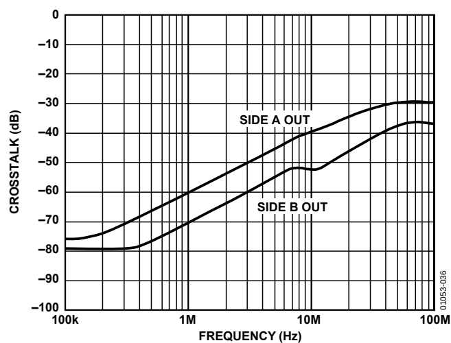
Figure 36. Output-to-Output Crosstalk vs. Frequency, V_S = \pm 2.5\text{ V}
