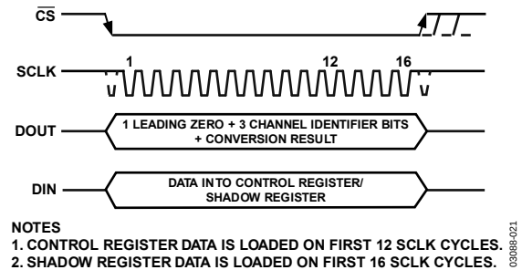
Figure 21. Normal Mode Operation
