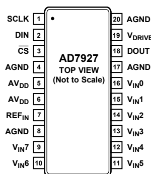
Figure 3. 20-Lead TSSOP Pin Configuration
