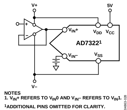
Figure 39. Pseudo Differential Inputs
