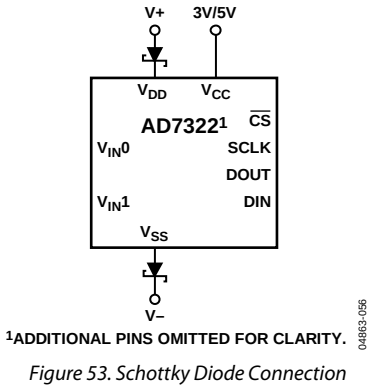
Figure 53. Schottky Diode Connection
