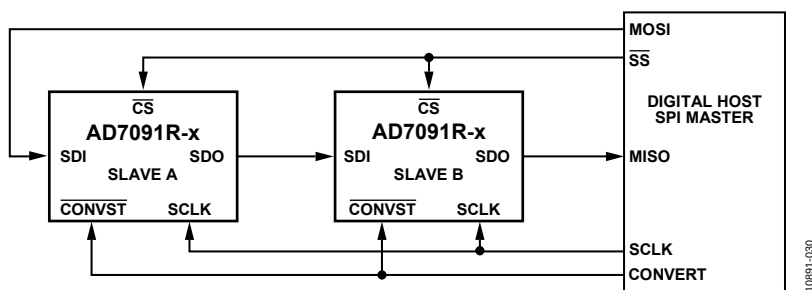
Figure 57. Daisy-Chain Configuration
