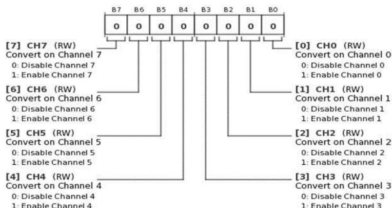
Figure 48. Channel Registers
