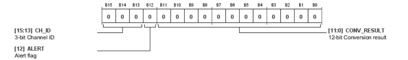
Figure 47. Conversion Result Register
