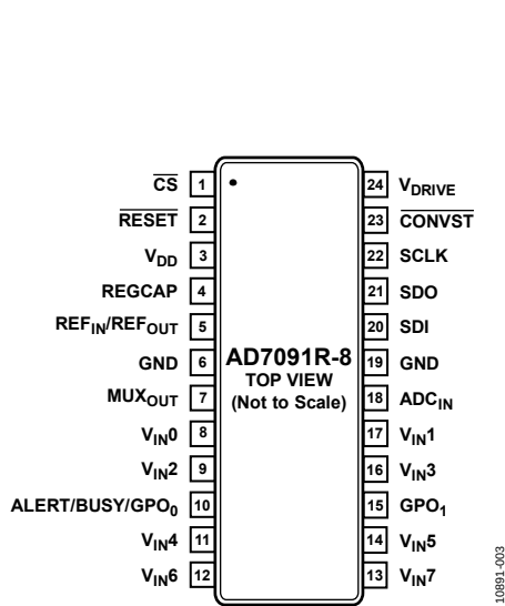
Figure 9. 8-Channel, 24-Lead TSSOP Pin Configuration
