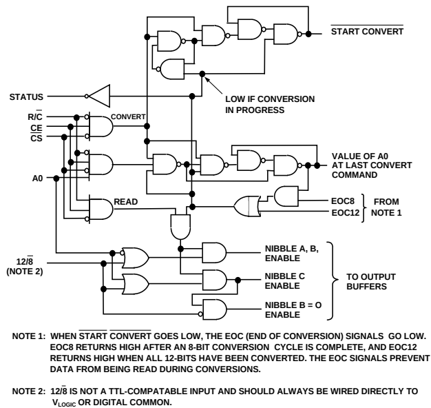
Figure 6. AD574A Control Logic
