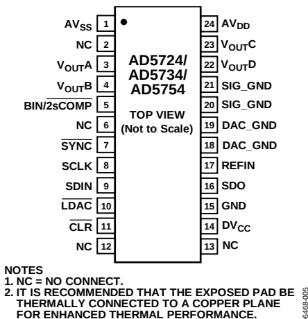
Figure 5. Pin Configuration
