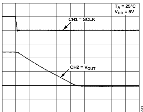
Figure 24. Midscale Settling Time
