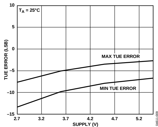
Figure 10. Total Unadjusted Error (TUE) vs. Supply at 25°C
