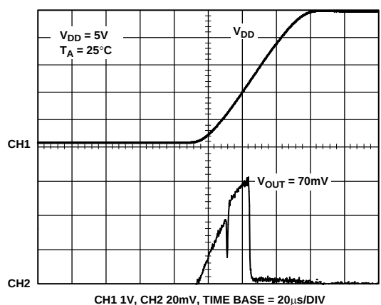
Figure 25. Power-On Reset to 0 V
