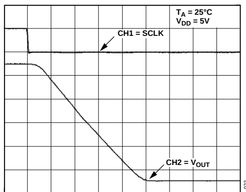
Figure 23. Full-Scale Settling Time
