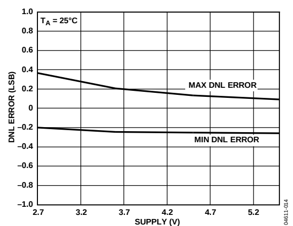
Figure 15. DNL Error vs. Supply at 25°C
