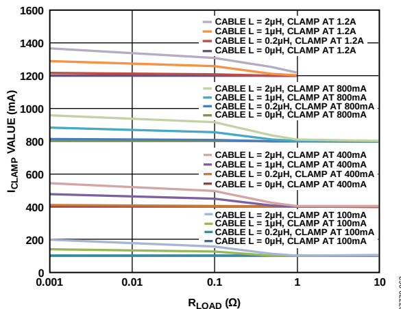
Figure 53. I_{CLAMP} Value vs. R_{LOAD} – Cal at 10hm
