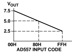
Figure 6. AD557 Input Code vs. Level Shifted Output in a “False” Ground Configuration
