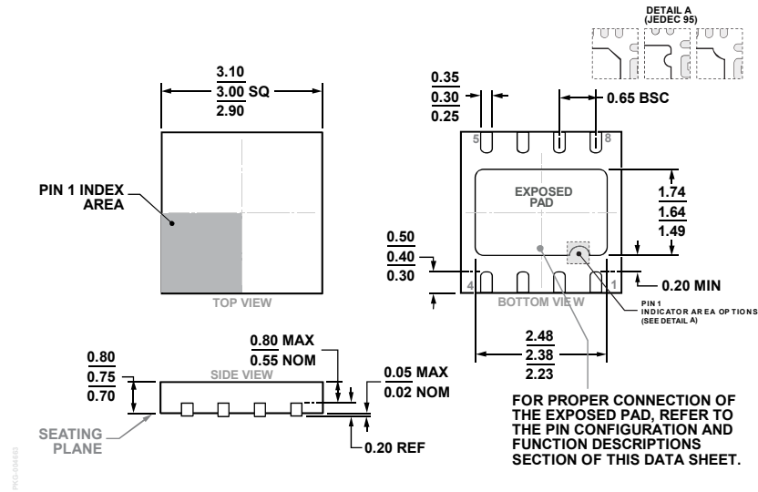
Figure 65. 8-Lead Lead Frame Chip Scale Package [LFCSP] 3 mm x 3 mm Body and 0.75 mm Package Height, Dual Lead (CP-8-3)
