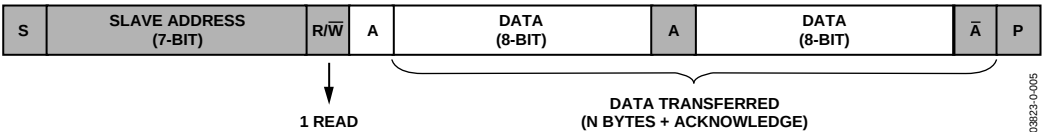
Figure 25. I 2 C—Master Reading Data from Slave
