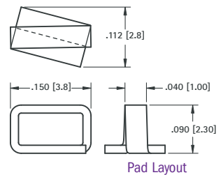
Pad Layout
