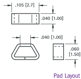
Pad Layout
