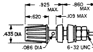
Mounting Detail
