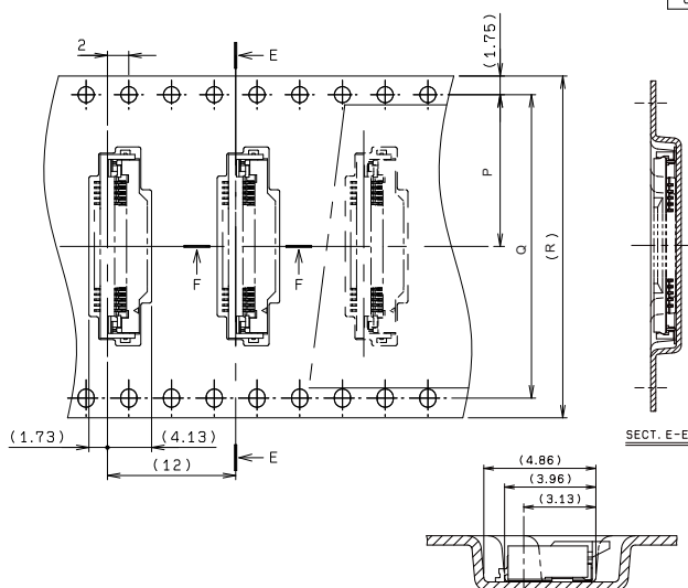
SECT. F-F
