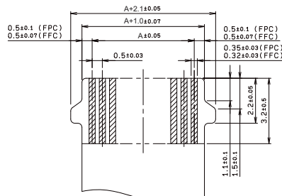
適用FPC/FFC寸法 APPLICABLE FPC/FFC
