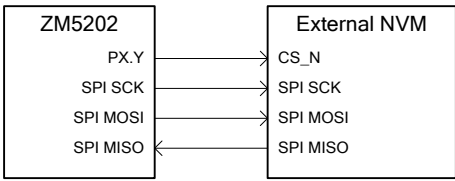
Figure 2.5: Typical interface to slave device
